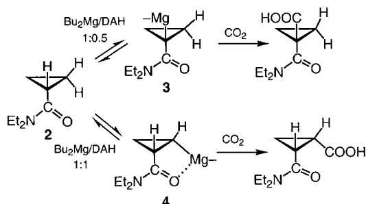
Scheme 2. Predominant position of magnesiation of 2 as a function of \text{Bu}_2\text{Mg} to DAH ratio. Standard conditions: heptane/THF (1:1); RT; two days; analysis after carboxylation at -78 \rightarrow 0^\circ\text{C} .
